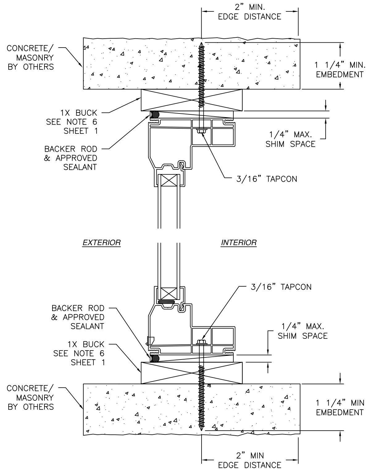
VERTICAL CROSS SECTION CONCRETE/MASONRY WITH 1X BUCK INSTALLATION FOR CONCRETE/MASONRY INSTALLATION WITHOUT 1X BUCK REFER TO JAMB INSTALLATION DETAILS
