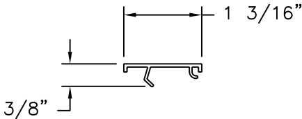
COMMON JAMB (037-R) FILL COVER EXTRUDED RIGID PVC
