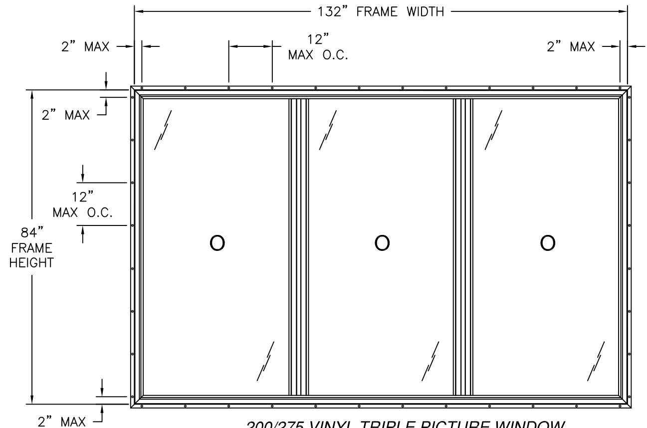
200/275 VINYL TRIPLE PICTURE WINDOW EXTERIOR VIEW FIN INSTALLATION
