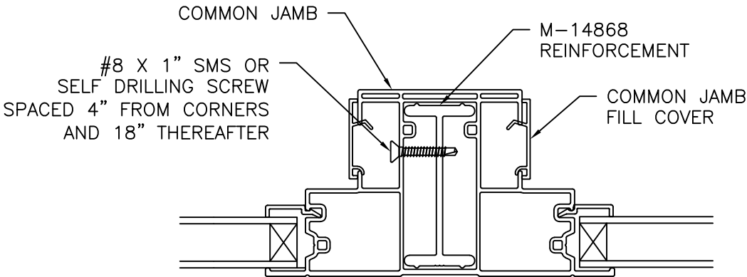
COMMON JAMB DETAIL
