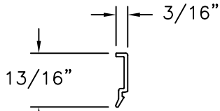
GLAZING BEAD (1703-R) EXTRUDED RIGID PVC
