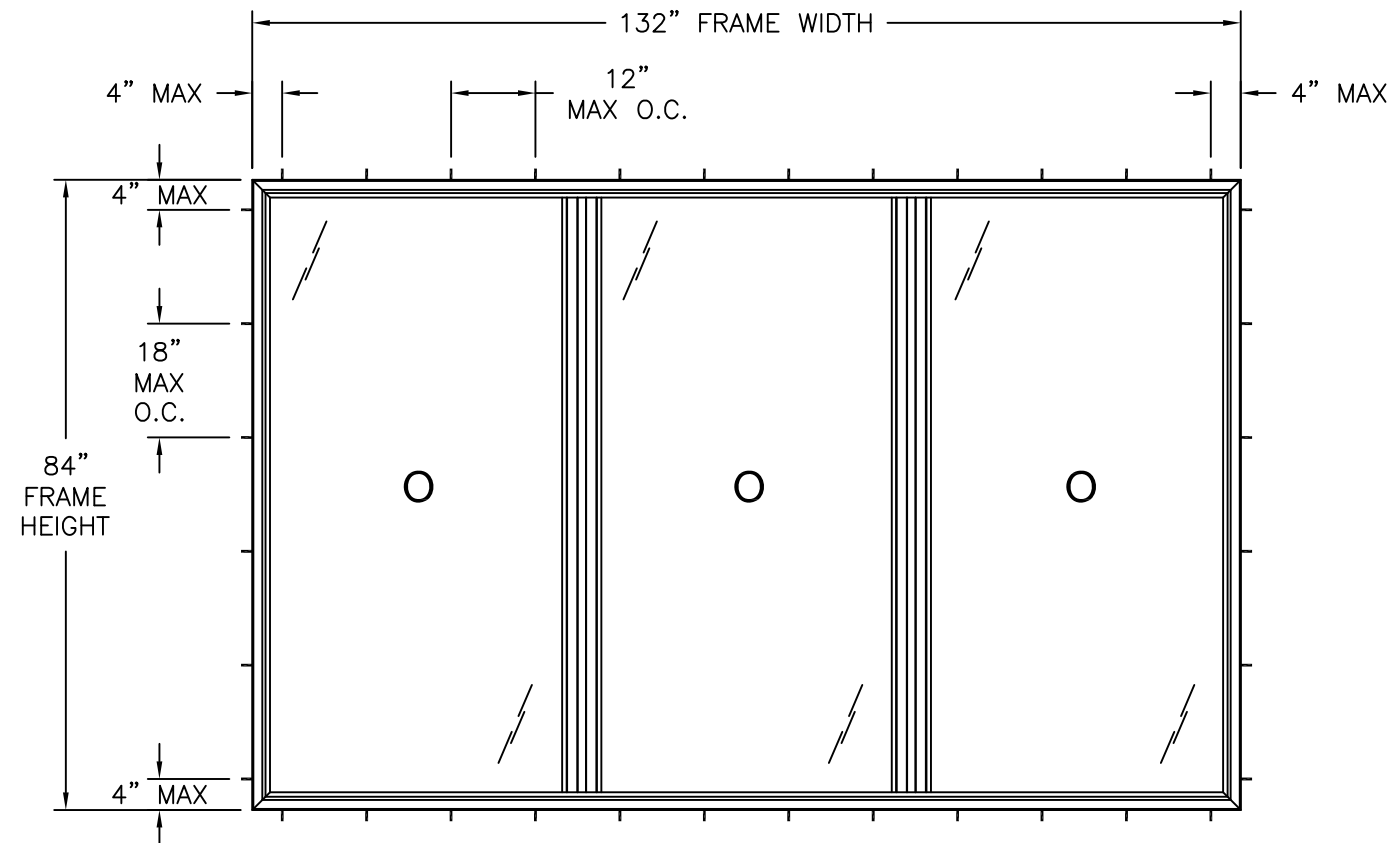
200/275 VINYL TRIPLE PICTURE WINDOW EXTERIOR VIEW FRAME INSTALLATION
